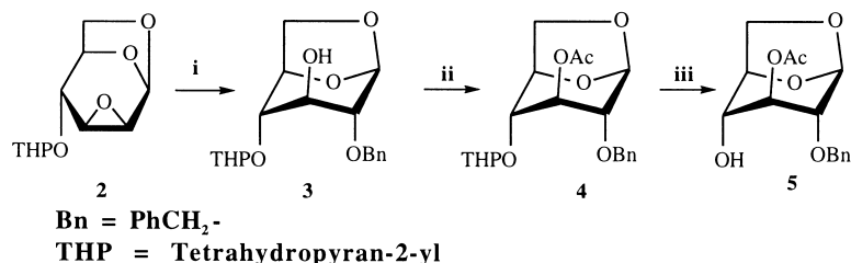
Scheme 1. Synthesis of the alcohol 5 . Reagents and conditions: (i) BnONa, BnOH, 110°C, 64%; (ii) Ac 2 O, Et 3 N, DMAP, CH 2 Cl 2 , 20°C; (iii) PTSA, MeOH, 20°C, 87% from 3 .
