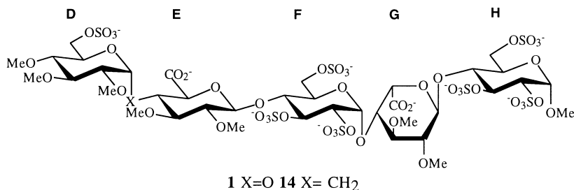
Figure 1. Structure of the synthetic O - and C -pentasaccharides.
