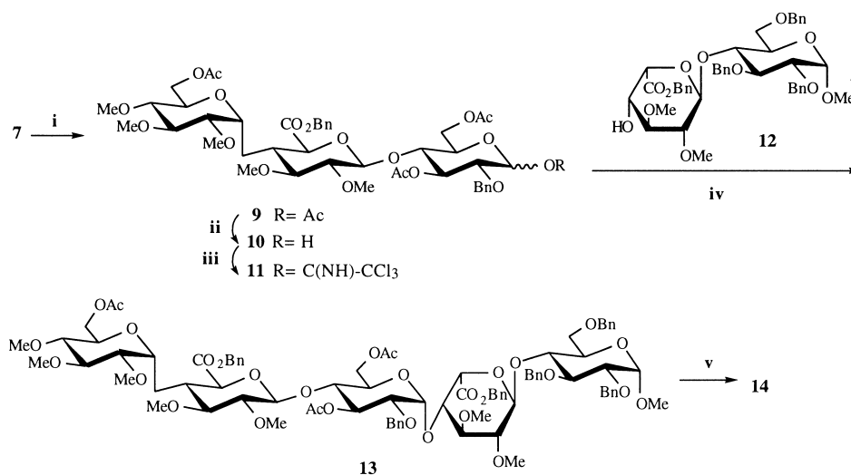
Scheme 3. Synthesis of the C -pentasaccharide 14 . Reagents and conditions: (i) H 2 SO 4 , AcOH, Ac 2 O, –20 °C, 100%; (ii) NH 3 NH 2 OAc, DMF, 90%; (iii) CCl 3 CN, DBU, CH 2 Cl 2 , 94%; (iv) TMSOTf, CH 2 Cl 2 , –20 °C, 79%; (v) 1. H 2 , Pd/C, CH 2 Cl 2 , MeOH, 99%, 2. NaOH, H 2 O, MeOH, 0 °C, 77%, 3. SO 3 , Et 3 N, DMF, 55 °C, 85%.
