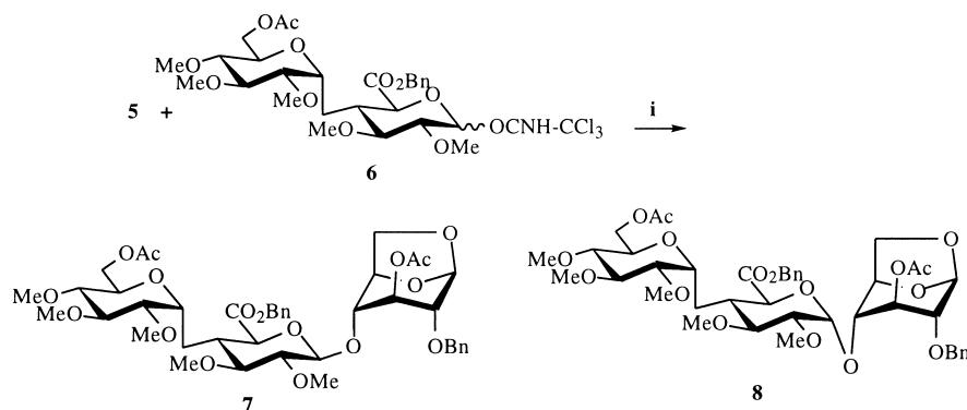
Scheme 2. Synthesis of the C -trisaccharide 8 . Reagent and conditions: TMSOTf, CH 3 CN, –37 °C, 88% 7:8 (5.5:1).
